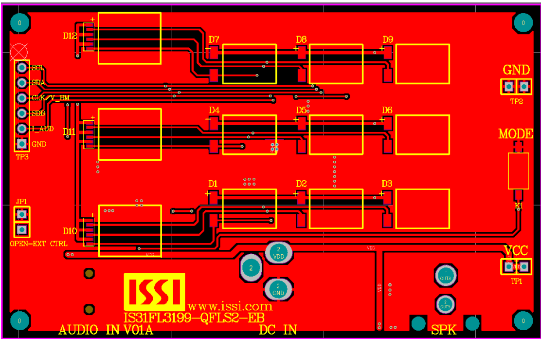
Figure 4: Board PCB Layout- Top Layer
