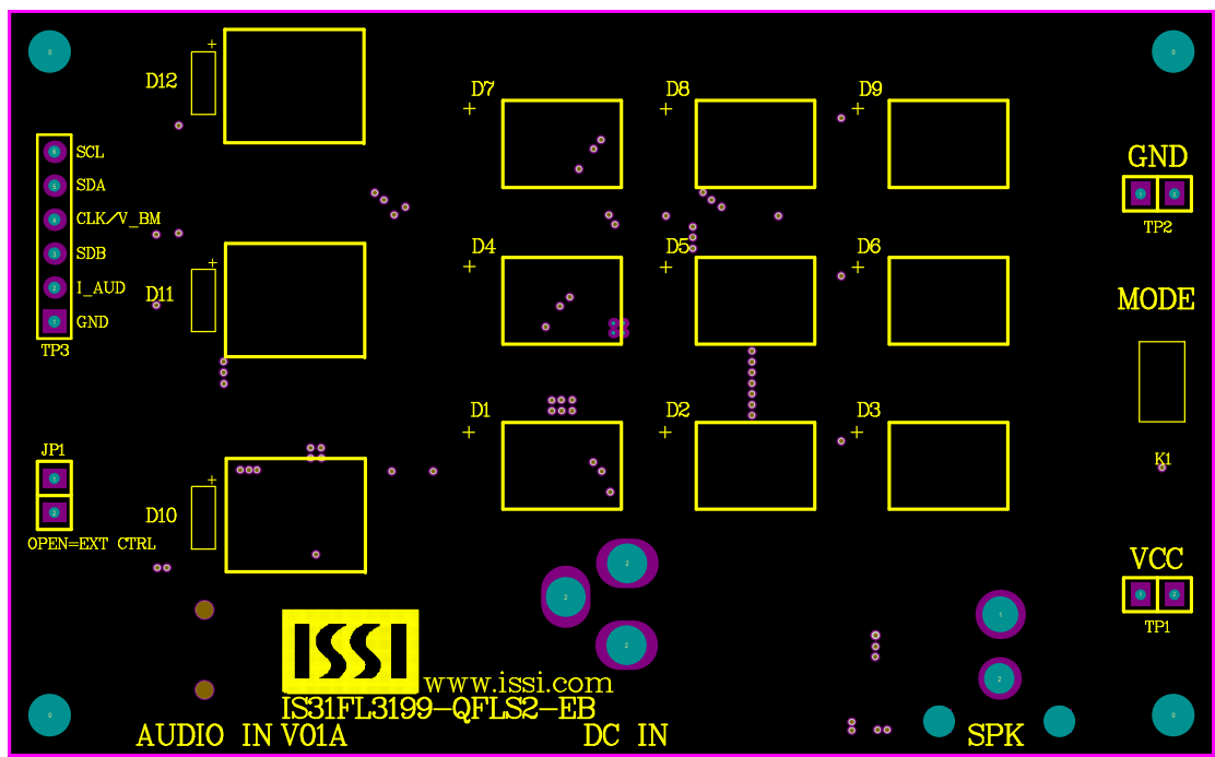
Figure 3: Board Component Placement Guide -Top Layer
