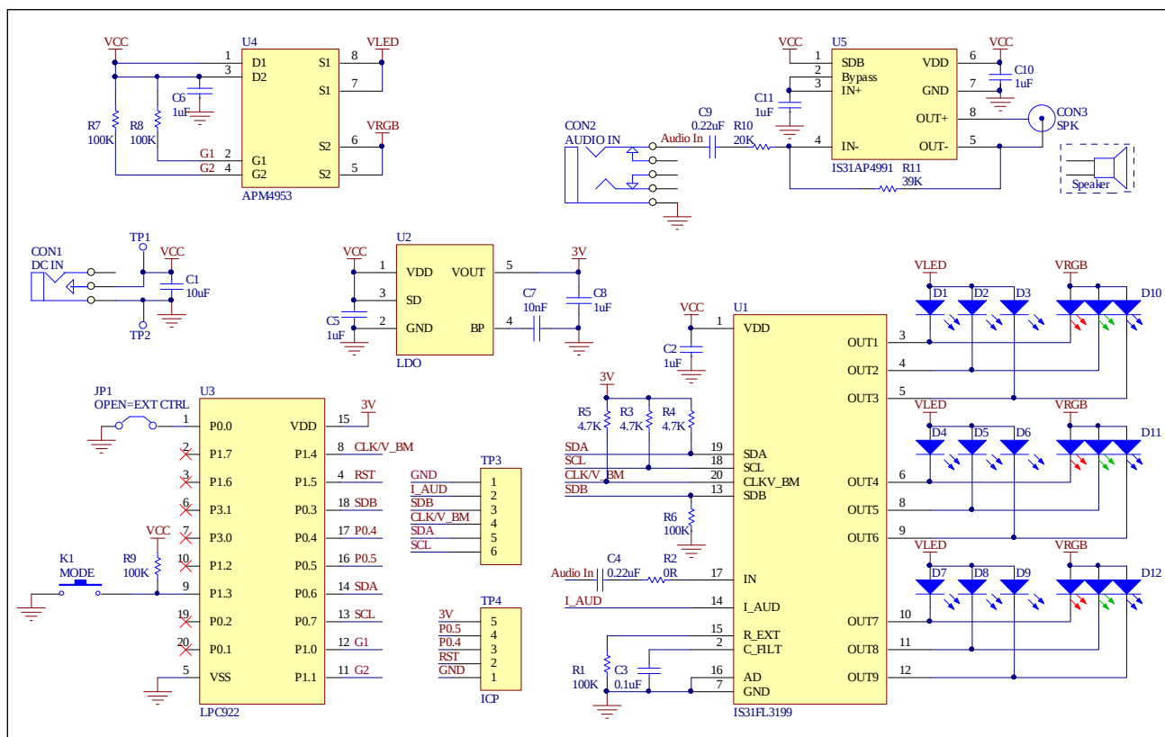
Figure 2: IS31FL3199 Application Schematic
