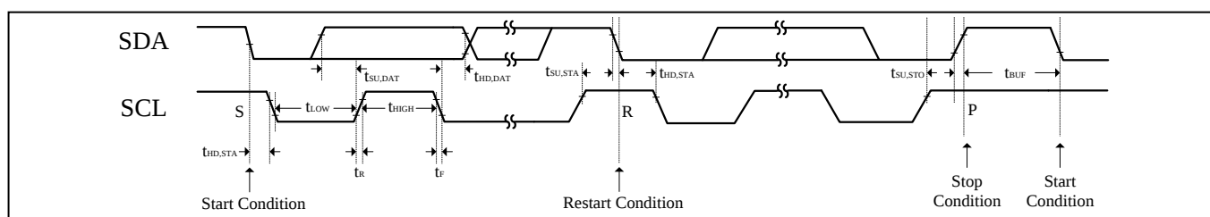
Figure 2 Interface timing
