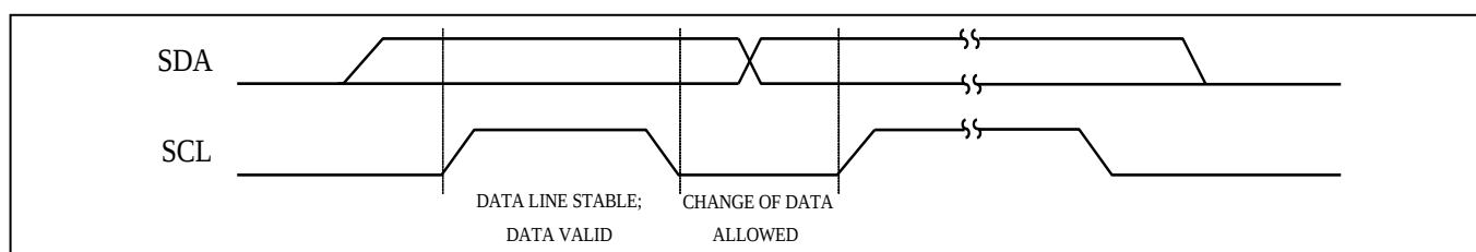
Figure 3 Bit transfer
