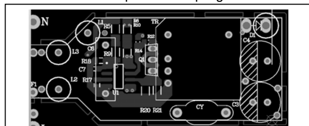
Figure 15 Typical PCB Top Layer
