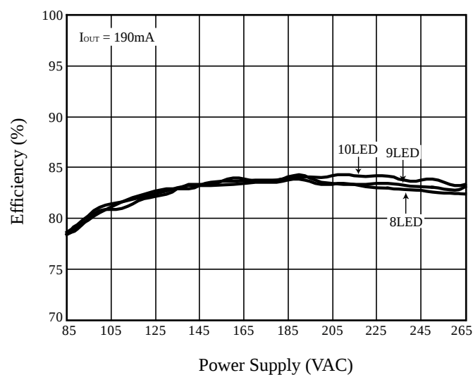
Figure 7 Efficiency vs. Power Supply
