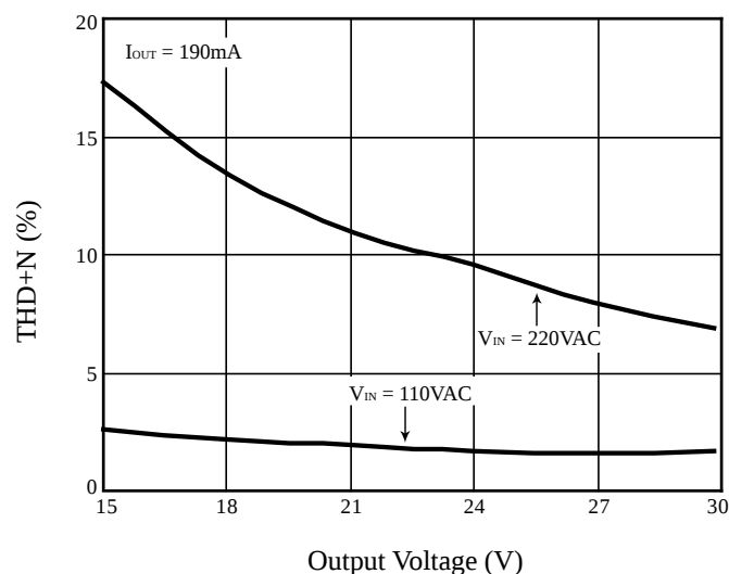
Figure 3 THD+N vs. Output Voltage
