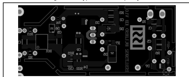
Figure 16 Typical PCB Bottom Layer
