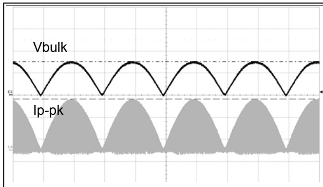
Figure 11 Active PFC
