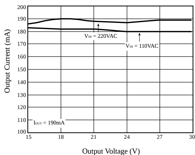
Figure 5 Output Current vs. Output Voltage
