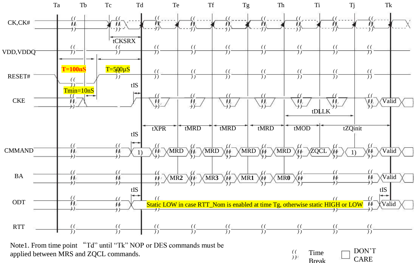
Figure2.1.2 Reset Procedure at Power Stable Condition
