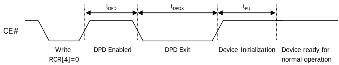
Figure 18: DPD Entry and Exit Timing Parameters
