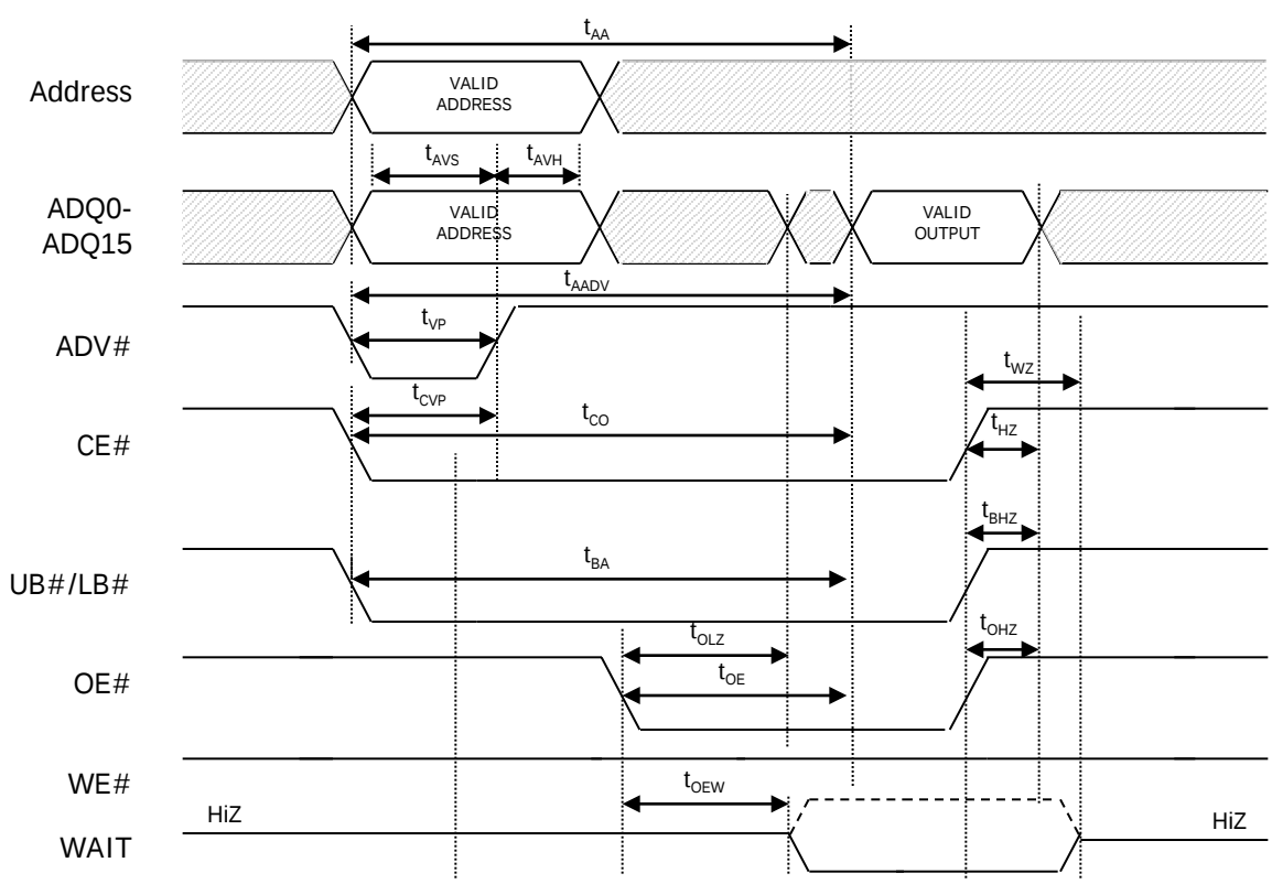
Figure 19: Asynchronous READ
