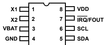
ISL1208 (8 LD TDFN) TOP VIEW
