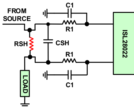
FIGURE 34. SIMPLIFIED FILTER DESIGN TO IMPROVE NOISE PERFORMANCE TO THE ISL28022
