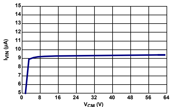
FIGURE 17. SHUNT I_{VIN} vs COMMON MODE VOLTAGE (MODE 5)
