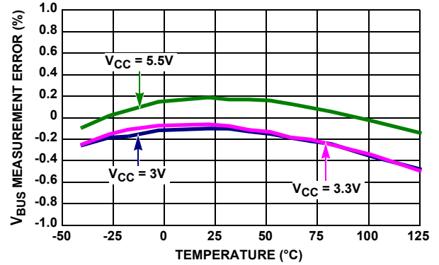
FIGURE 10. V_{BUS} MEASUREMENT ERROR vs TEMPERATURE
