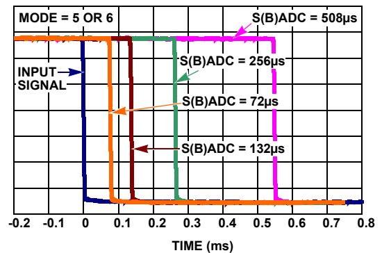
FIGURE 26. INTERRUPT TIMING
