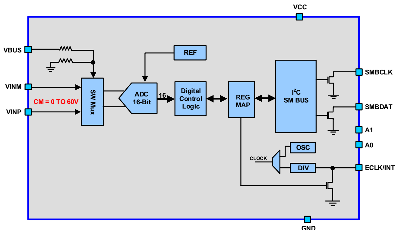
FIGURE 2. BLOCK DIAGRAM
