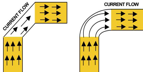
FIGURE 44. AVOID ROUTING ORTHOGONAL CONNECTIONS FOR TRACES THAT HAVE HIGH CURRENT FLOWS
