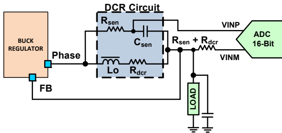
FIGURE 41. A SIMPLIFIED CIRCUIT EXAMPLE OF A DCR
