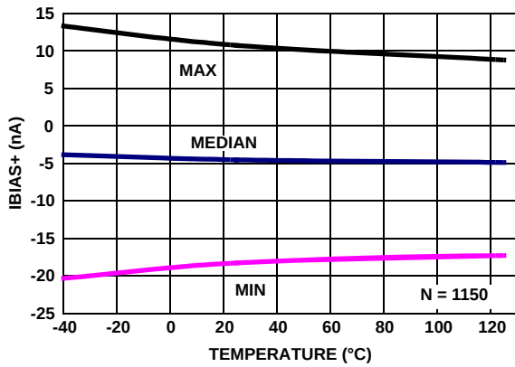
FIGURE 26. I_{BIAS+} vs TEMPERATURE, V_+ , V_- = \pm 1.2V
