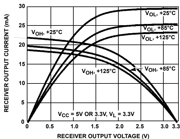
FIGURE 7. RECEIVER OUTPUT CURRENT vs RECEIVER OUTPUT VOLTAGE
