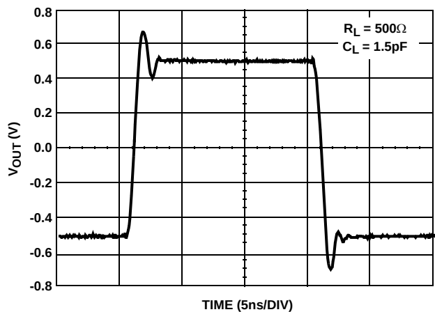
FIGURE 5. TRANSIENT RESPONSE
