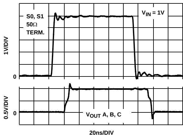
FIGURE 9. CHANNEL TO CHANNEL TRANSIENT RESPONSE ( V_{IN} = 1V )
