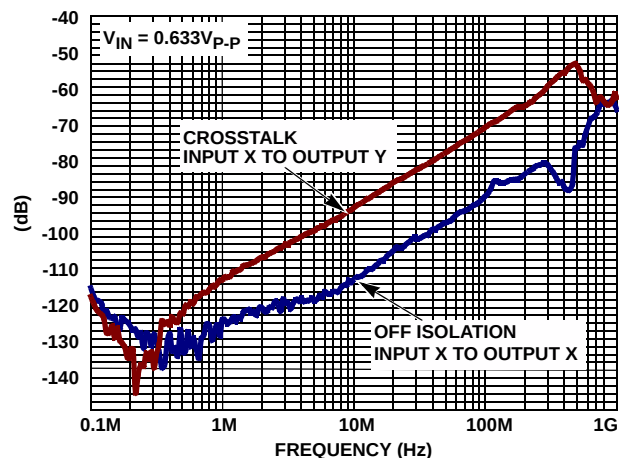
FIGURE 6. CROSSTALK AND OFF ISOLATION
