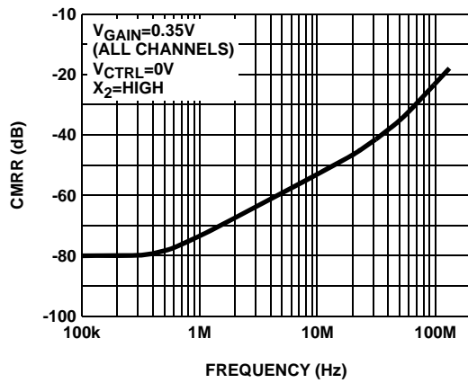
FIGURE 11. COMMON-MODE REJECTION
