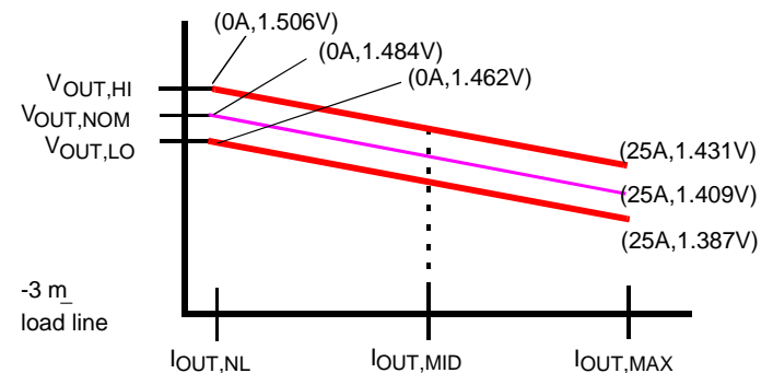
FIGURE 11. IMVP-IV™ AND IMVP-IV+™ ACTIVE MODE STATIC LOAD LINE
