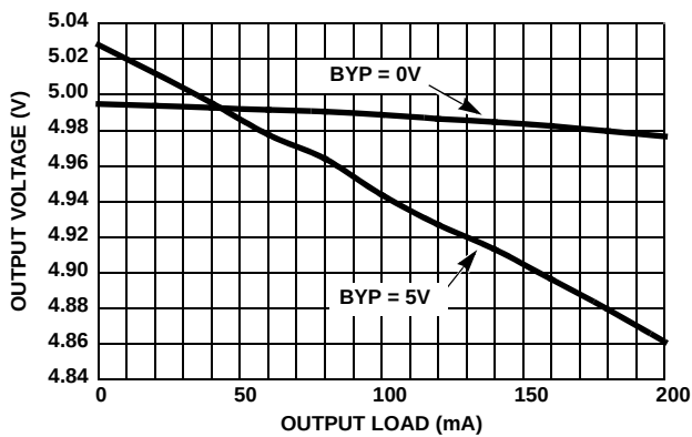
FIGURE 29. LDO OUTPUT 5V vs LOAD
