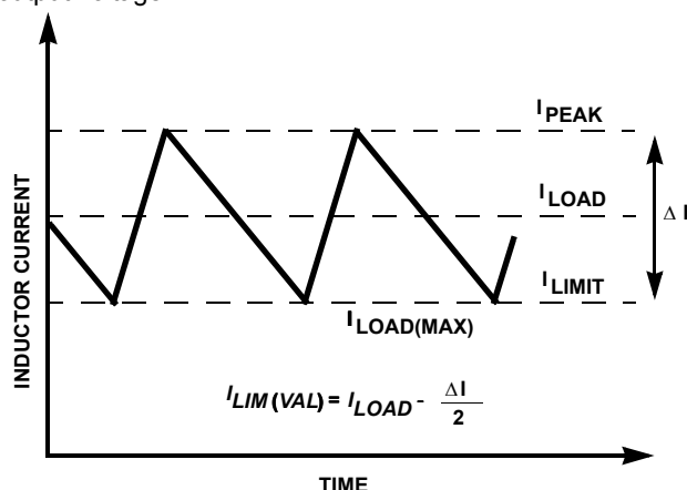
FIGURE 73. "VALLEY" CURRENT LIMIT THRESHOLD POINT
