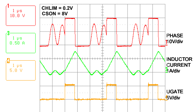
FIGURE 12. SWITCHING WAVEFORMS AT DIODE EMULATION
