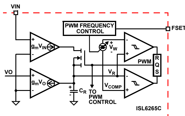
FIGURE 6. MODULATOR CIRCUITRY
