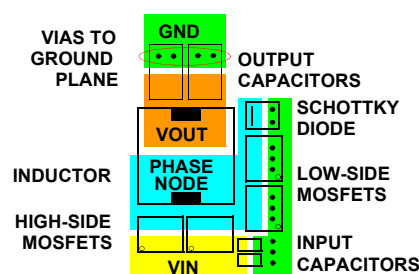
FIGURE 14. TYPICAL POWER COMPONENT PLACEMENT
