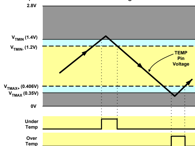
FIGURE 21. CRITICAL VOLTAGE LEVELS FOR TEMP PIN
