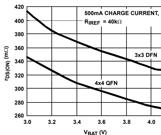
FIGURE 10. r_{DS(ON)} vs OUTPUT VOLTAGE USING CURRENT LIMITED ADAPTERS
