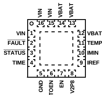
ISL6298 (16 LEAD QFN)
