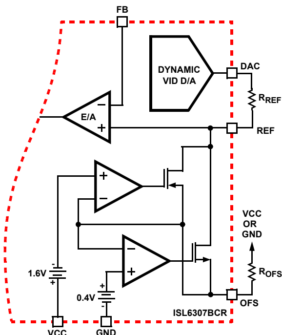
FIGURE 9. OUTPUT VOLTAGE OFFSET PROGRAMMING WITH ISL6307B
