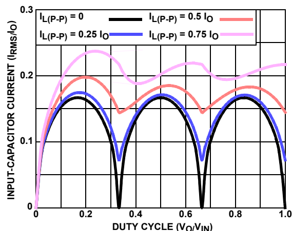
FIGURE 24. NORMALIZED INPUT-CAPACITOR RMS CURRENT vs DUTY CYCLE FOR 3-PHASE CONVERTER
