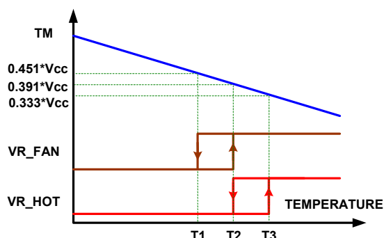
FIGURE 19. VR_HOT AND VR_FAN SIGNAL vs TM VOLTAGE Based on the NTC temperature characteristics and the desired threshold of the VR_HOT signal, the pull-up resistor R TM1 of TM
