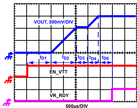
FIGURE 14. SOFT-START WAVEFORMS
