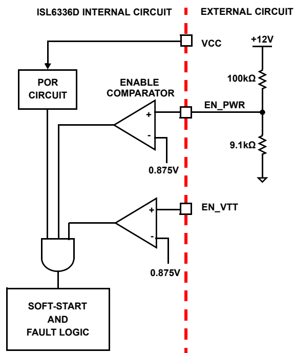
FIGURE 13. POWER SEQUENCING USING THRESHOLD SENSITIVE ENABLE (EN) FUNCTION
