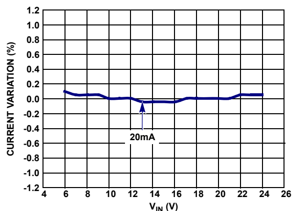
FIGURE 6. CURRENT REGULATION
