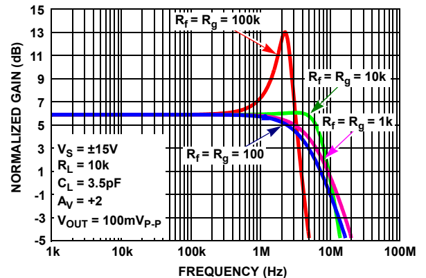
FIGURE 37. SIMULATED CLOSED LOOP GAIN vs R_f/R_g
