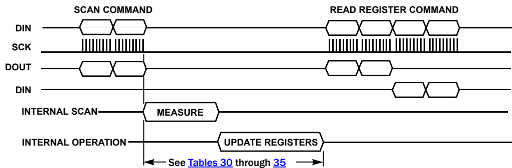
FIGURE 64. SCAN/MEASURE COMMAND TIMING WITH RESPONSE (STAND-ALONE)
