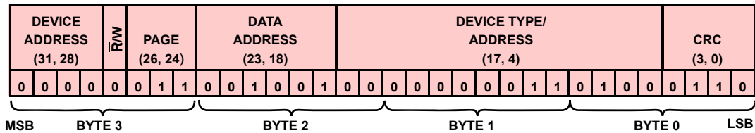
FIGURE 63C. DEVICE COMMUNICATIONS ADMINISTRATION RESPONSE: IDENTIFY, DEVICE 4, MIDDLE STACK DEVICE
