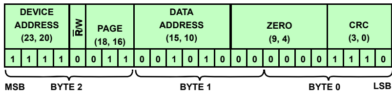
FIGURE 62A. DEVICE LEVEL COMMAND: SLEEP
