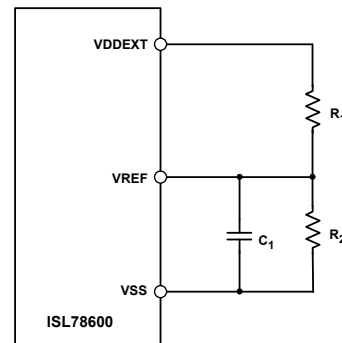
FIGURE 50. CELL READING ACCURACY ADJUSTMENT SYSTEM
