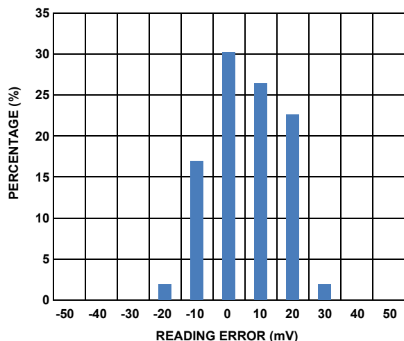
FIGURE 8. INITIAL PACK VOLTAGE ACCURACY AT 39.6V, +25°C HISTOGRAM
