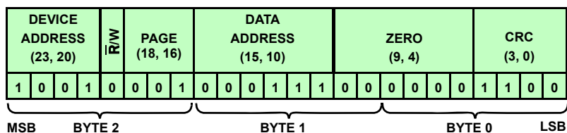
FIGURE 62D. DEVICE READ: DEVICE 9, GET CELL 7 DATA
