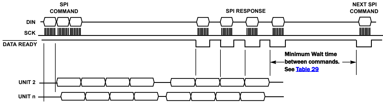
FIGURE 70. MINIMUM WAIT BETWEEN COMMANDS (DAISY CHAIN RESPONSE - TOP DEVICE)
