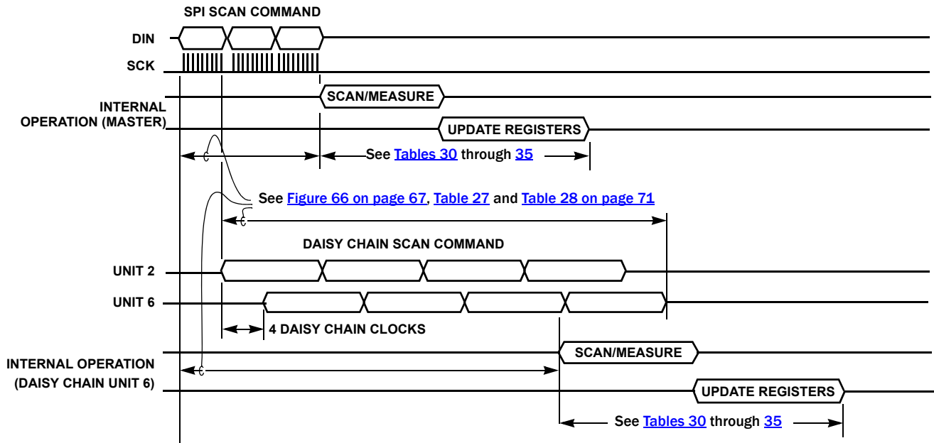
FIGURE 65. MEASUREMENT TIMING (6 DEVICE DAISY CHAIN)
