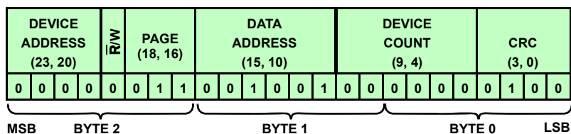
FIGURE 62F. IDENTIFY COMMAND
