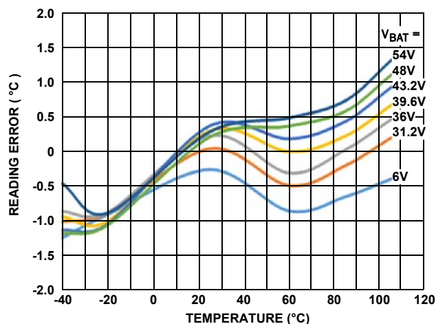
FIGURE 9. IC TEMPERATURE ERROR vs TEMPERATURE
