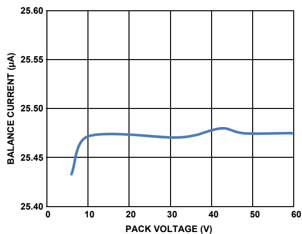
FIGURE 12. BALANCE CURRENT vs PACK VOLTAGE
