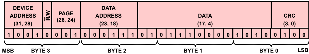
FIGURE 63A. DEVICE DATA RESPONSE: DEVICE 9, CELL 7 VOLTAGE = 14'h170A (3.6V)
