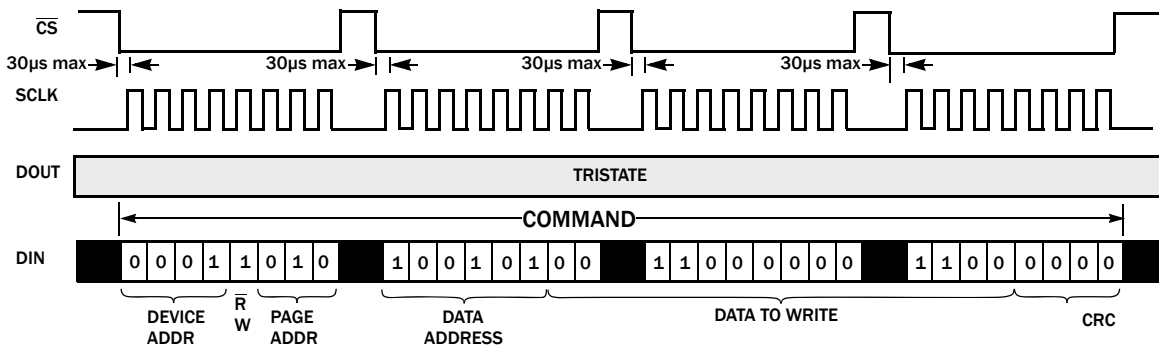
FIGURE 61. SPI HALF DUPLEX (DAISY CHAIN) WRITE REGISTER COMMAND EXAMPLE: WRITE DEVICE 1, DEVICE SETUP REGISTER
