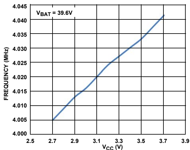
FIGURE 19. 4MHz OSCILLATOR FREQUENCY vs VCC
