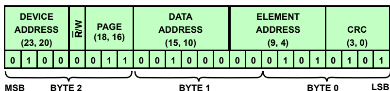
FIGURE 62E. ELEMENT LEVEL COMMAND: DEVICE 4, MEASURE CELL 5 VOLTAGE
