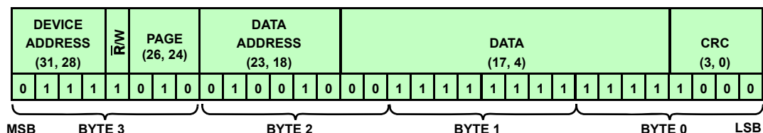
FIGURE 62G. DEVICE WRITE: DEVICE 7, WRITE EXTERNAL TEMPERATURE LIMIT = 14'h0FFF
