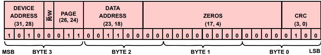
FIGURE 63B. DEVICE COMMUNICATIONS ADMINISTRATION RESPONSE: DEVICE 10, ACK
