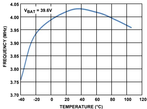
FIGURE 18. 4MHz OSCILLATOR FREQUENCY vs TEMPERATURE
