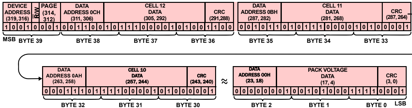
FIGURE 63D. DEVICE DATA RESPONSE: DEVICE 9, READ ALL CELL VOLTAGE DATA
