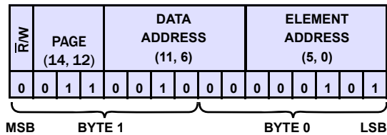
FIGURE 56D. DEVICE LEVEL COMMAND: MEASURE CELL 5 VOLTAGE
