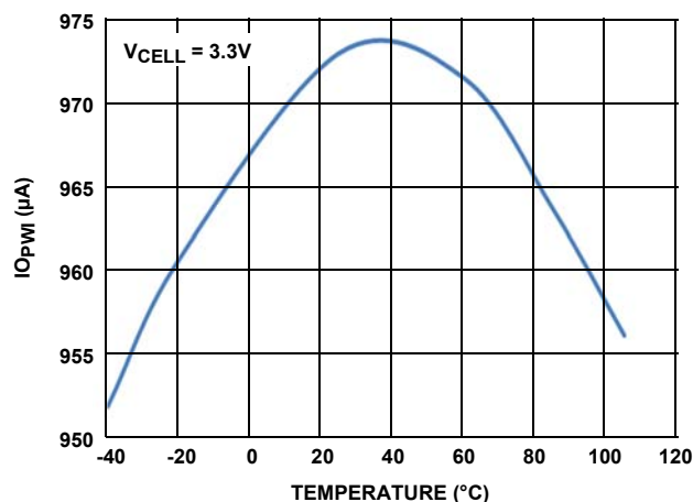
FIGURE 14. OPEN-WIRE TEST CURRENT vs TEMPERATURE (1mA SETTING)
