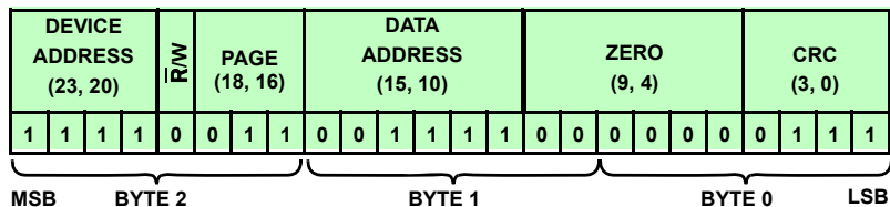
FIGURE 62B. DEVICE LEVEL COMMAND: WAKEUP
