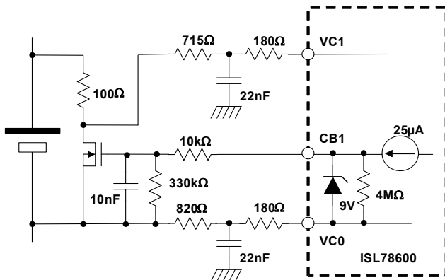
FIGURE 35. CELL MONITOR AND BALANCE CIRCUIT ARRANGEMENT (VC1)
