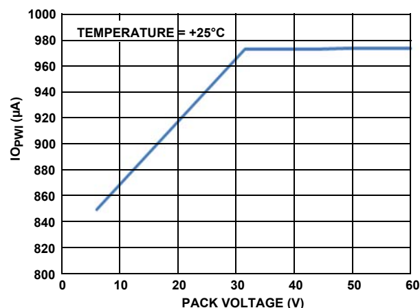
FIGURE 15. OPEN-WIRE TEST CURRENT vs PACK VOLTAGE (1mA SETTING)
