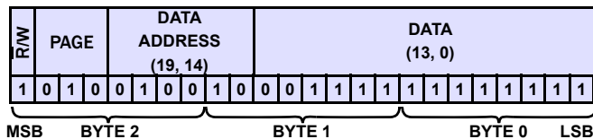
FIGURE 56E. DEVICE WRITE: WRITE EXTERNAL TEMPERATURE
