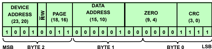
FIGURE 62C. DEVICE LEVEL COMMAND: DEVICE 9, SCAN VOLTAGES
