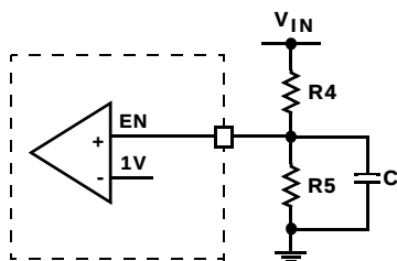
FIGURE 38. EXTERNAL RESISTOR DIVIDER
