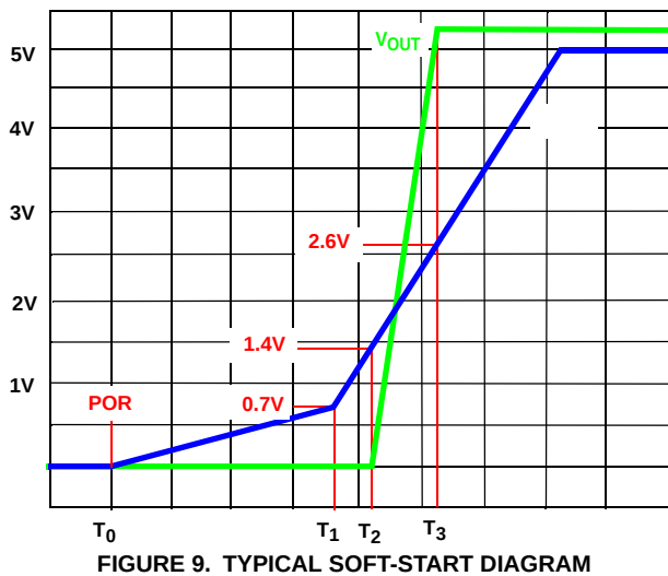
FIGURE 9. TYPICAL SOFT-START DIAGRAM
