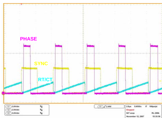
FIGURE 11. SYNCHRONIZATION OPERATION
