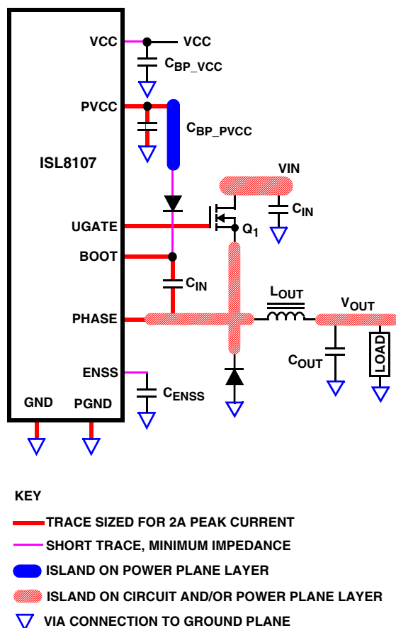
FIGURE 17. PRINTED CIRCUIT BOARD POWER PLANES AND ISLANDS
