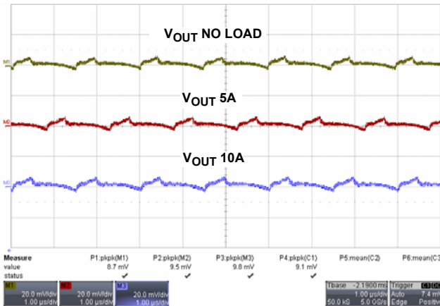
FIGURE 20. 3.3V OUTPUT RIPPLE
