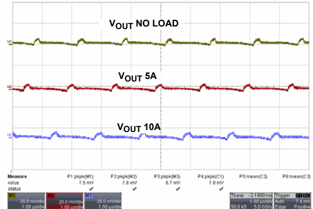
FIGURE 18. 1.5V OUTPUT RIPPLE
