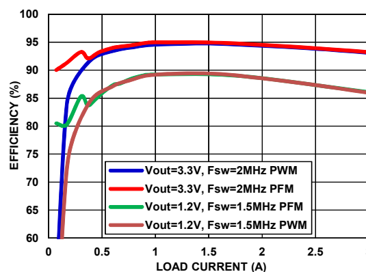
FIGURE 2. EFFICIENCY vs LOAD 5V_{IN}
