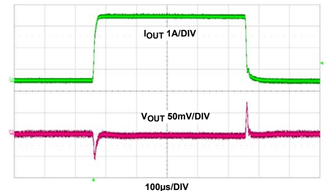
FIGURE 15. V_{IN} = 5V , V_{OUT} = 1.2V , I_{OUT} = 0 TO 3A , f_{SW} = 1.5MHz , C_{OUT} = 2 \times 22\mu F CERAMIC CAPACITORS
