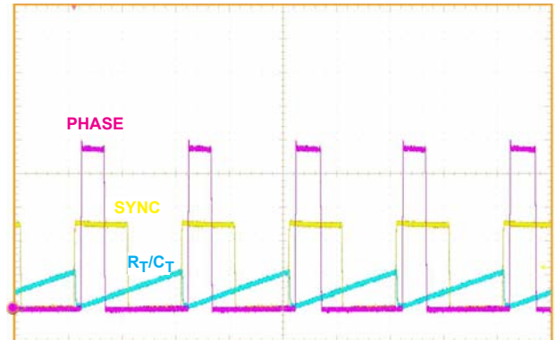
FIGURE 20. SYNCHRONIZATION OPERATION
