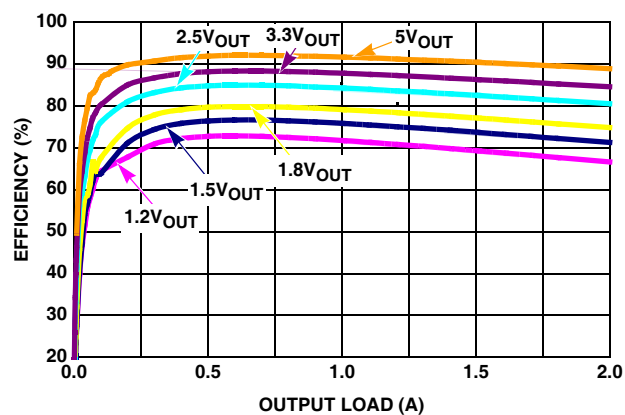
FIGURE 3. EFFICIENCY vs LOAD, 12\text{V}_{IN}
