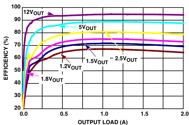
FIGURE 4. EFFICIENCY vs LOAD, 25\text{V}_{IN}
