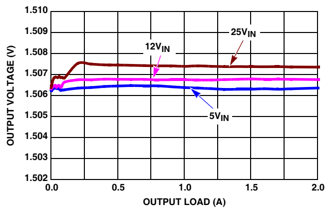
FIGURE 7. V_{OUT} REGULATION vs LOAD, 1.5\text{V}_{OUT}
