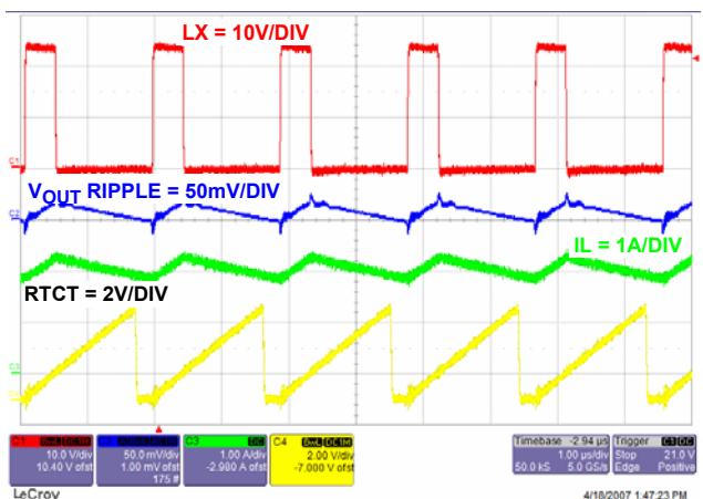
FIGURE 20. STEADY STATE OPERATION WITH FULL LOAD
