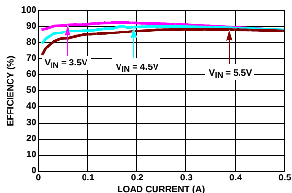
FIGURE 4. EFFICIENCY vs LOAD CURRENT ( V_{OUT} = 2.5\text{V} )
