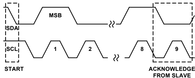
Figure 22. Acknowledge on the SMBus
