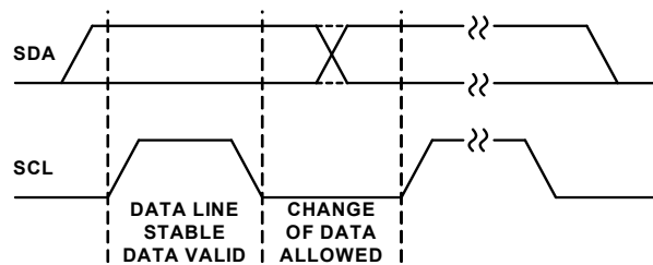
Figure 20. Data Validity
