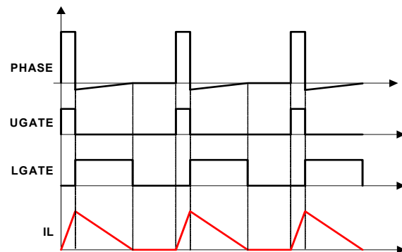
Figure 27. Diode Emulation
