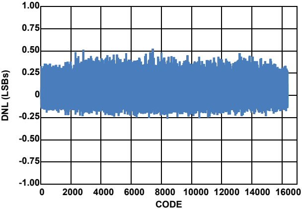
FIGURE 9. DIFFERENTIAL NONLINEARITY
