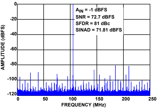
FIGURE 13. SINGLE-TONE SPECTRUM @ 105MHz
