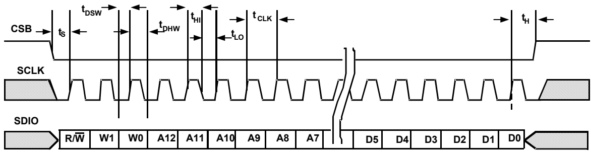
SPI WRITE
