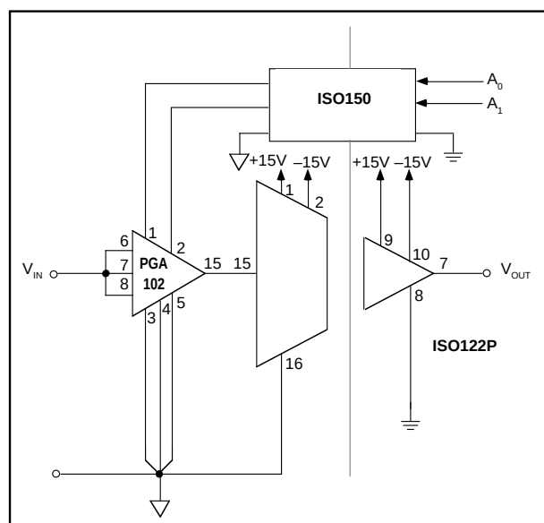
FIGURE 3. Programmable-Gain Isolation Channel with Gains of 1, 10, and 100.
