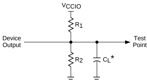
Figure 9. Test Load
