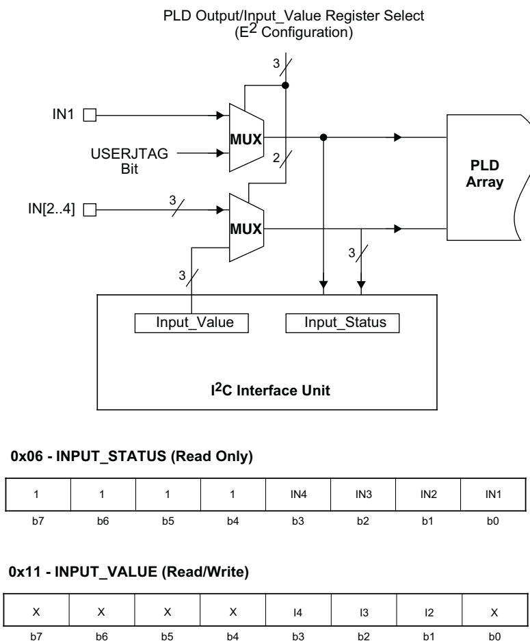
Figure 20. I 2 C Digital Input Interface
