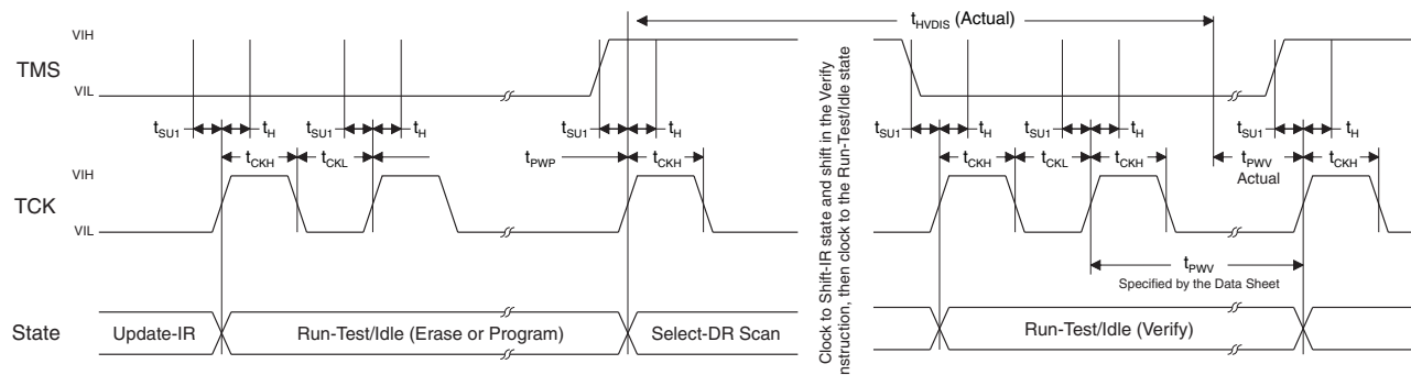
Figure 6. Discharge Timing Diagram
