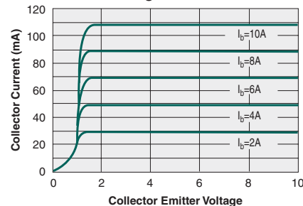
Typical Transfer Characteristics of Darlington Transistor
