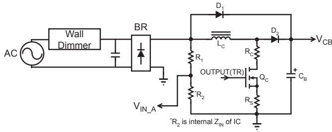
Figure 9.5 : Chopping Schematic
