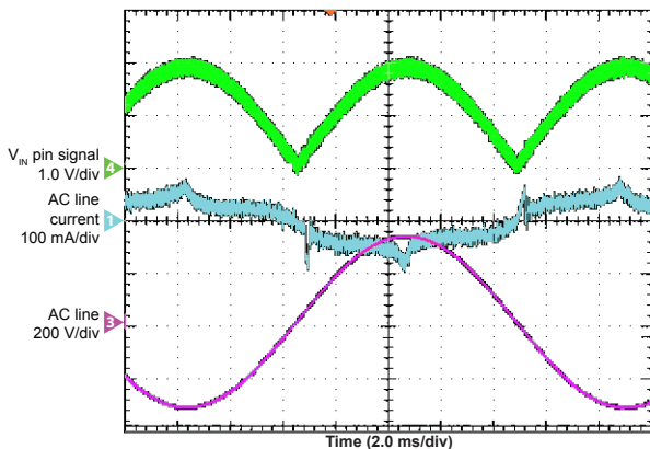
Figure 10.5 : No Dimmer
