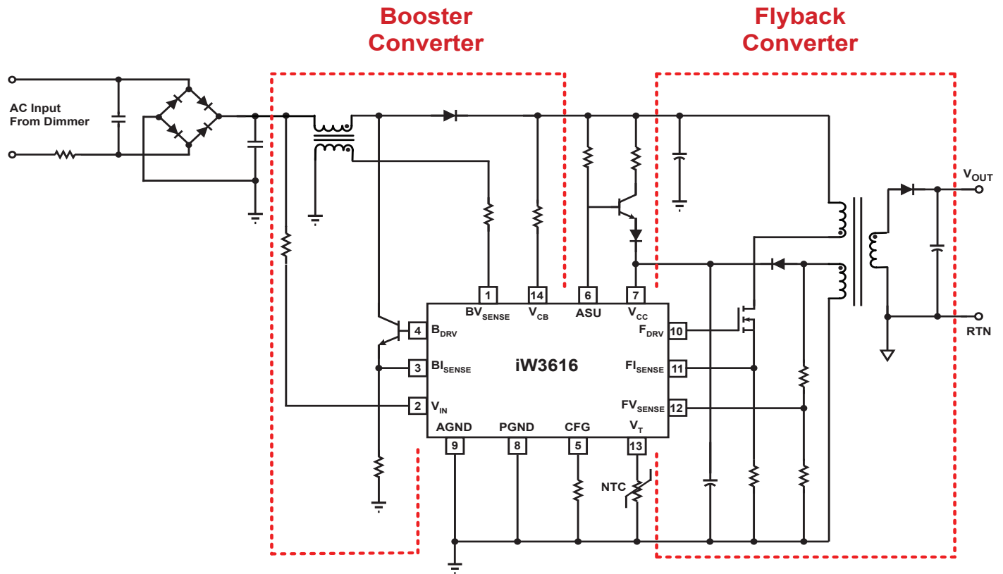
Figure 3.1 : iW3616 Simplified Schematic
