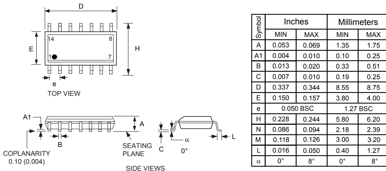
Figure 6.1 : Physical dimensions, 14-lead SOIC package
