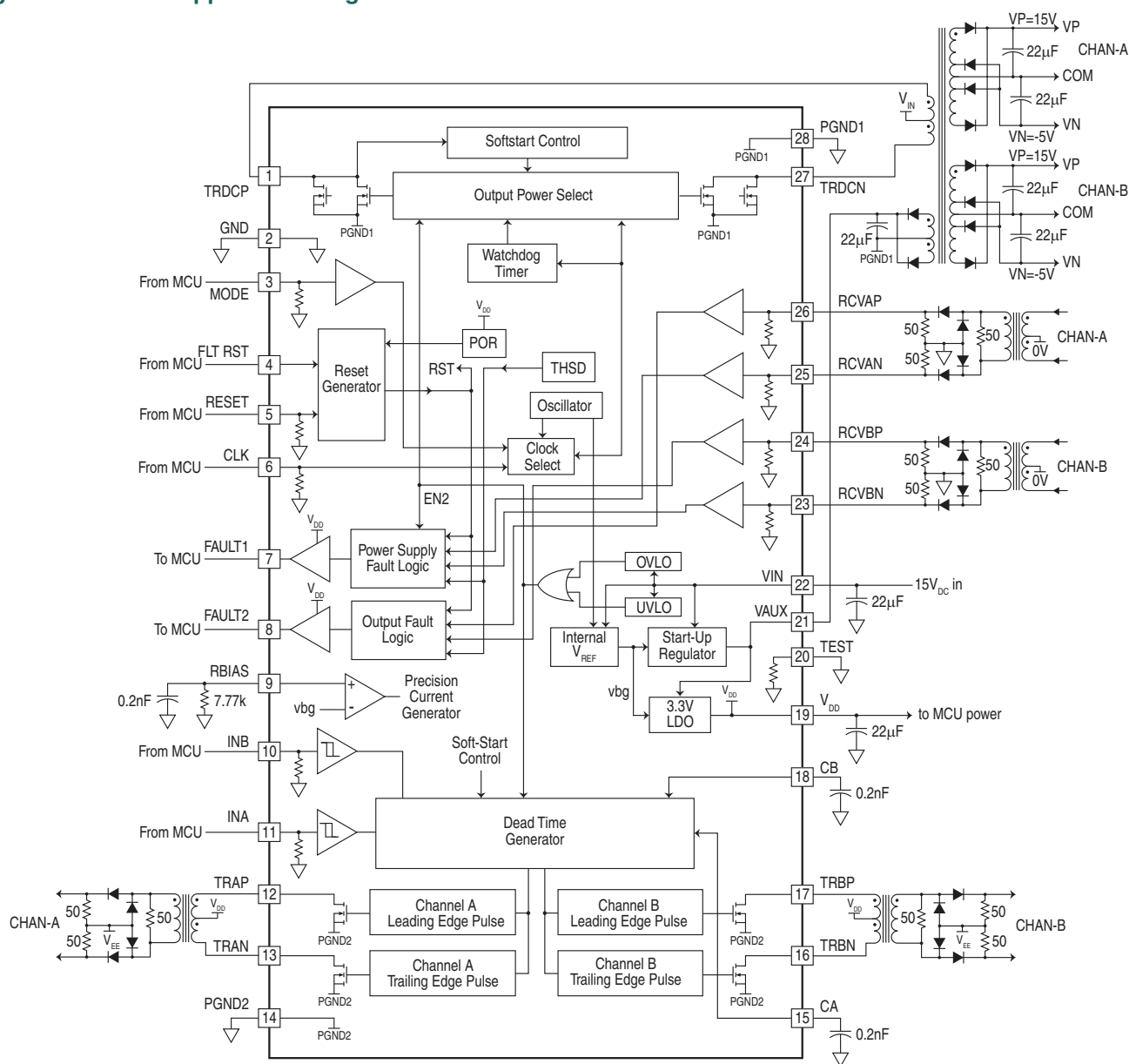
Figure 12 IX6610 Application Diagram
