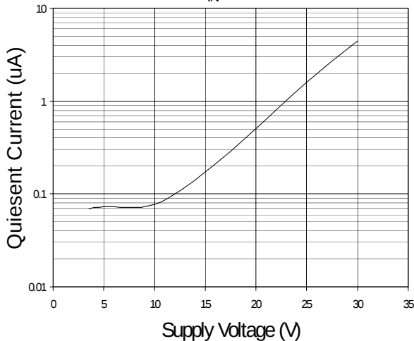
Fig. 14 Quiescent Current vs. Supply Voltage V_{\text{IN}} = 0\text{V}
