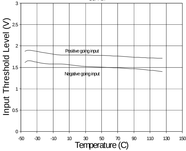
Fig. 10 Input Threshold Levels vs. Temperature V_{\text{SUPPLY}} = 15\text{V}
