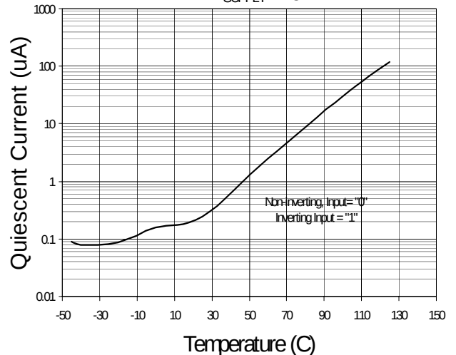
Fig. 15 Quiescent Current vs. Temperature V_{\text{SUPPLY}} = 15\text{V}
