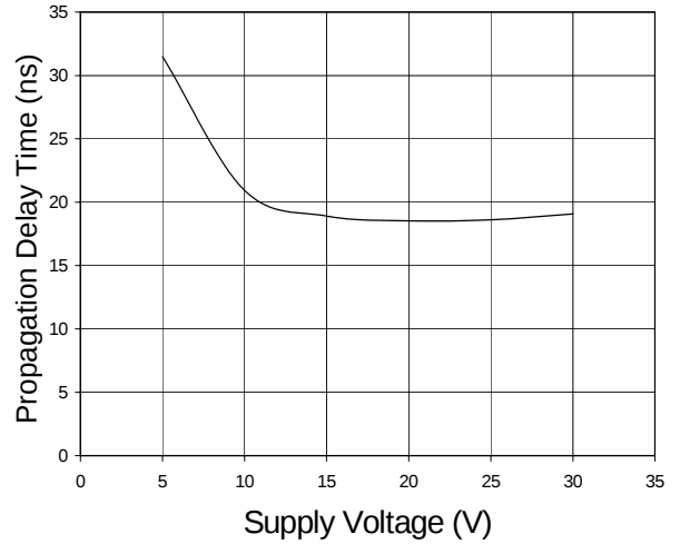
Fig. 11 Propagation Delay vs. Supply Voltage Rising Input, C_{\text{LOAD}} = 1000\text{pF}
