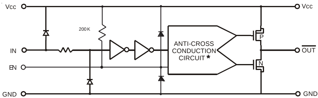
Figure 2 - IXDE514 Inverting 14A Gate Driver Functional Block Diagram
