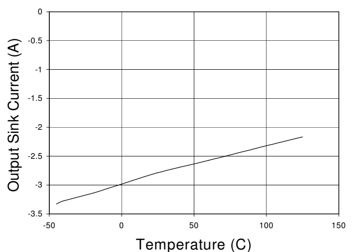
Output Sink Current vs. Temperature V_{SUPPLY} = 15V
