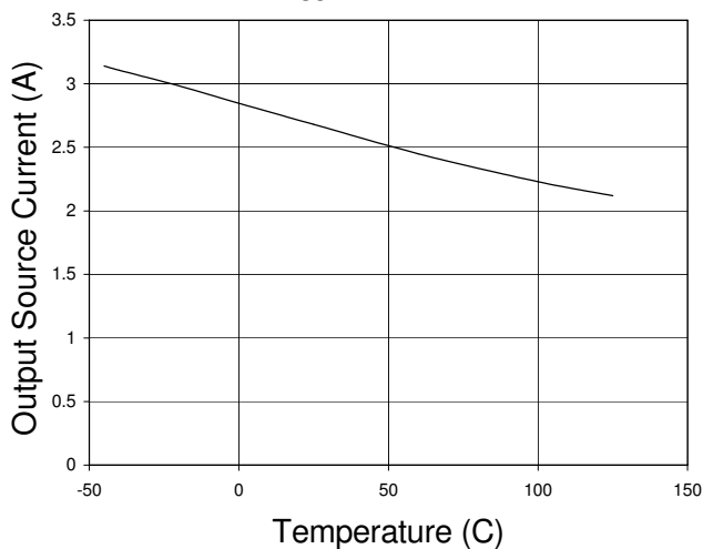
Output Source Current vs. Temperature V_{SUPPLY} = 15V
