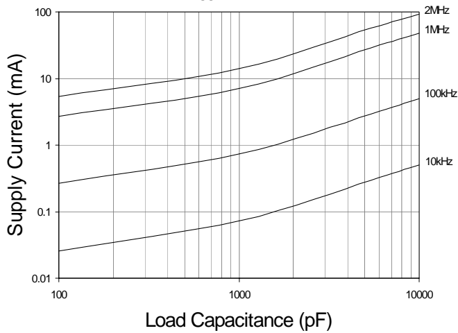
Supply Current vs. Capacitive Load V_{\text{SUPPLY}} = 5V
