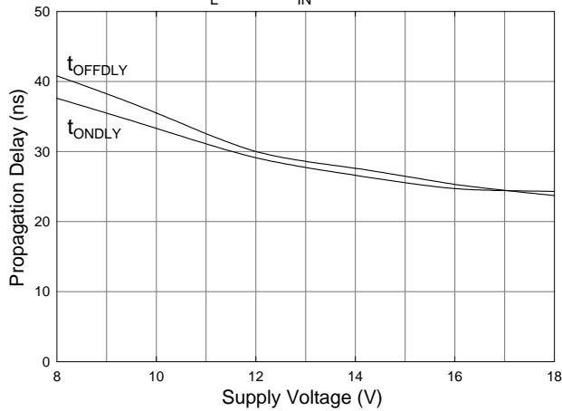
Fig. 17 Propagation Delay vs. Supply Voltage C_L=15\text{nF} V_{IN}=5\text{V}@1\text{kHz}
