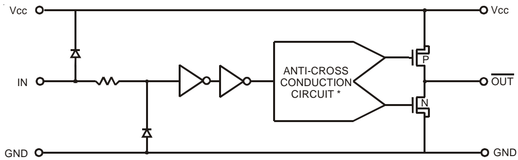
Figure 1 - IXDI514 Inverting 14A Gate Driver Functional Block Diagram
