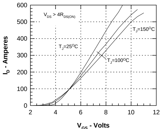
Figure 3. Admittance Curves
