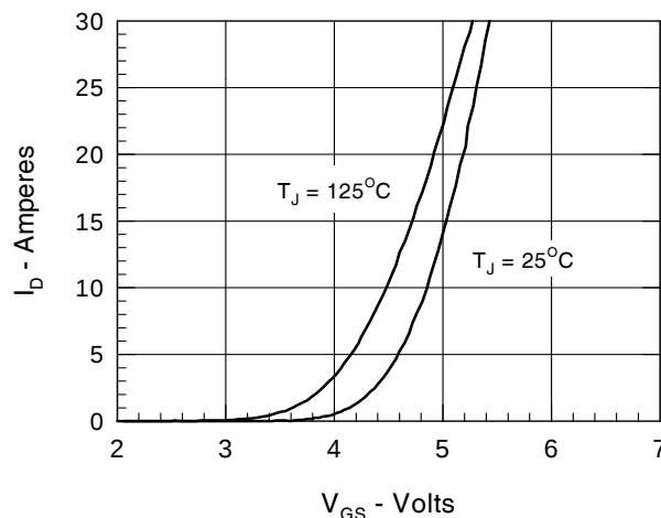
Figure 4. Admittance Curves
