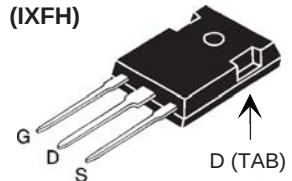
TO-3P (IXFQ)
