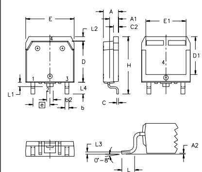
TO-268 Outline
