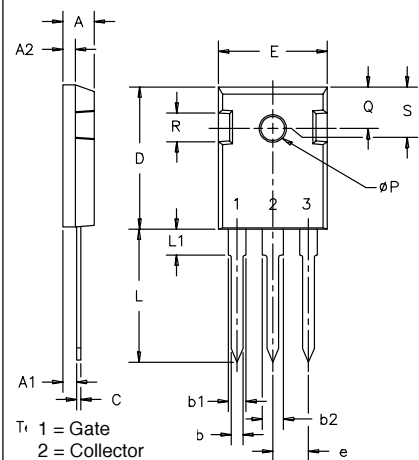
Tab = Collector
