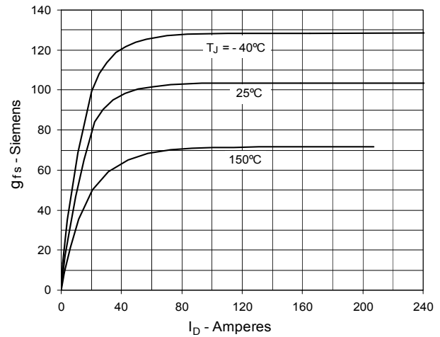
Fig. 8. Transconductance
