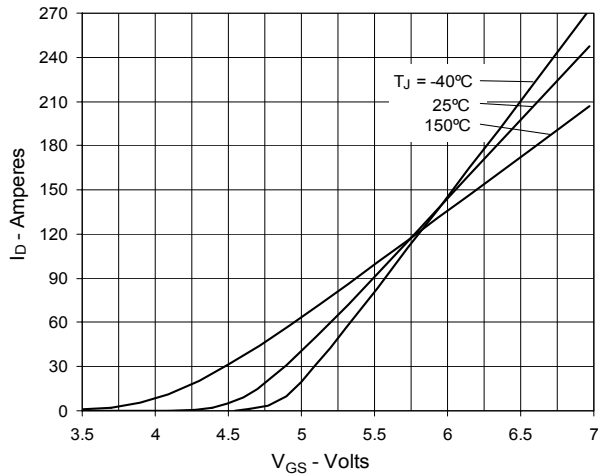
Fig. 7. Input Admittance
